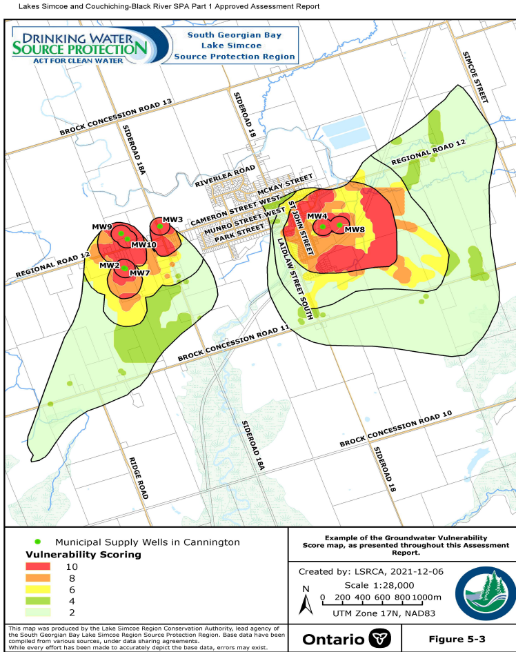
Figure 5–3: Example of the Groundwater Vulnerability Score map, as presented throughout this Assessment Report
