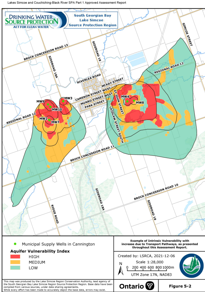
Figure 5–2: Example of Intrinsic Vulnerability with increase due to Transport Pathways, as presented throughout this Assessment Report
