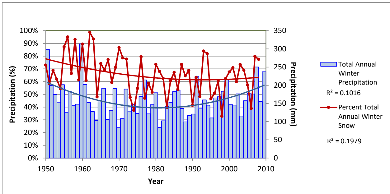
Figure 20-15: Percentage of Annual Winter Precipitation (snow) vs. Total Annual Winter Precipitation at the Alliston-Nelson Meteorological Monitoring Station.
