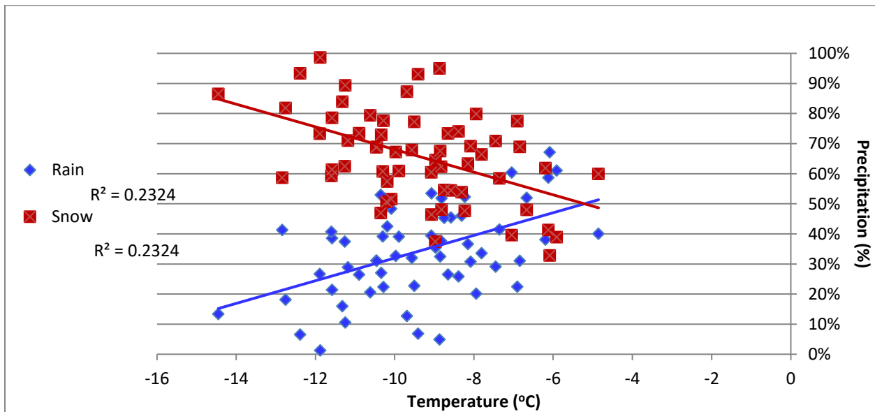
Figure 20-16: Percentage Annual Winter Precipitation (rain & snow) Vs. Average Annual Winter Temperature at the Alliston-Nelson Meteorological Monitoring Station.
