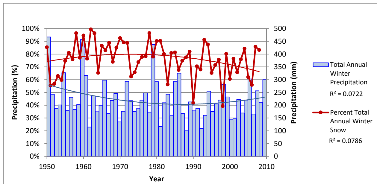
Figure 20-17: Percentage of Annual Winter Precipitation (snow) vs. Total Annual Winter Precipitation at the Barrie WPCC Meteorological Monitoring Station.
