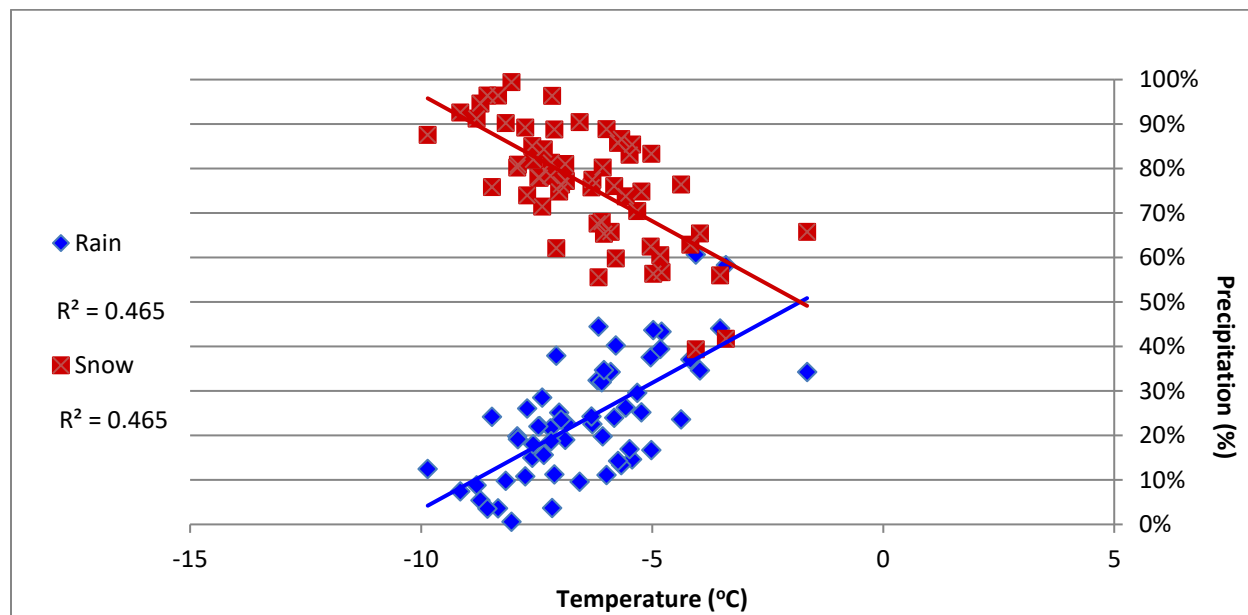
Figure 20-18 Percentage Annual Winter Precipitation (rain & snow) Vs. Average Annual Winter Temperature at the Barrie WPCC Meteorological Monitoring Station.
