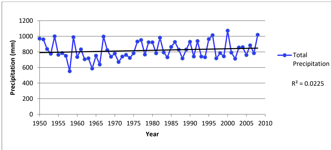
Figure 20-13: Total Annual Precipitation at the Alliston-Nelson Meteorological Monitoring Station.
