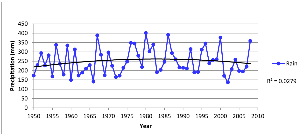
Figure 20-19: Total Annual Summer Precipitation (rain) at the Alliston-Nelson Meteorological Monitoring Station.
