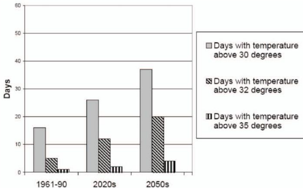
Figure 20-8: Past and future projection of hot days in the City of Toronto (Source: Environment Canada, 2002).
