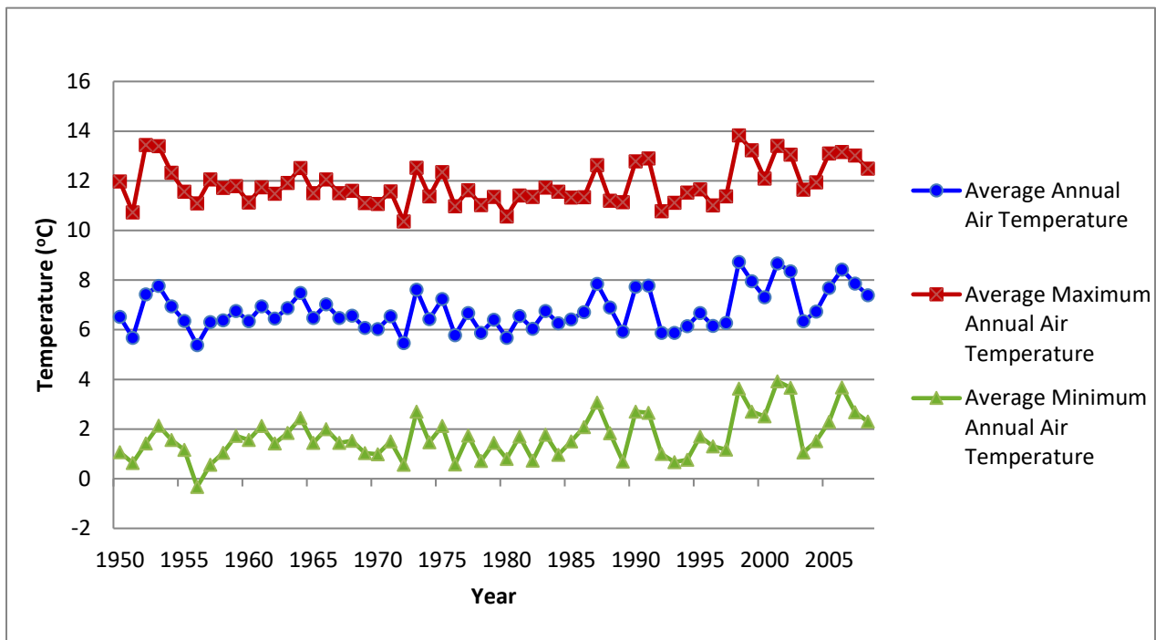
Figure 20-11: Comparison of the Average Annual, Maximum and Minimum Temperatures at the Barrie WPC Meteorological Monitoring Station.
