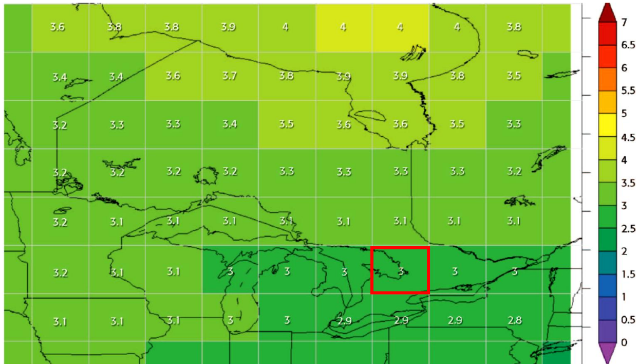
Figure 20-2: Projected increase in average annual temperature (°C) in the 2050's compared with 1961-1990 under High GHG emissions (CCCSN, 2009). Area highlighted in red roughly corresponds to the Source Protection Region.
