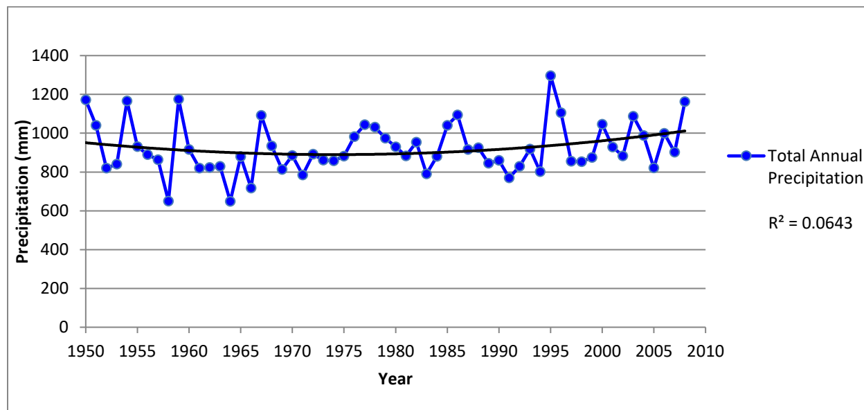
Figure 20-14: Total Annual Precipitation at the Barrie WPCC Meteorological Monitoring Station.
