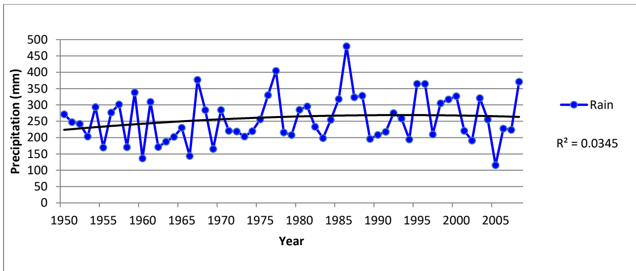
Figure 20-20: Total Annual Summer Precipitation at Barrie WPCC Meteorological Monitoring Station.
