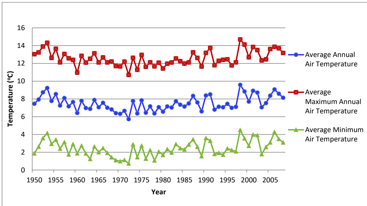
Figure 20-9: Comparison of the Average Annual, Maximum and Minimum Temperatures at the Alliston-Nelson Monitoring Station.
