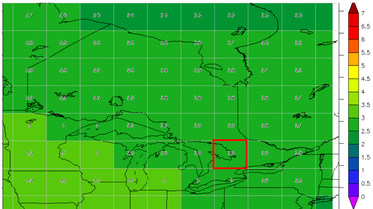
Figure 20-4: Projected change in average SUMMER air temperature (°C) over Ontario for 2050s compared with 1961-1990 under HIGH GHG emissions (CCCSN, 2009). Area highlighted in red roughly corresponds to the Source Protection Region.
