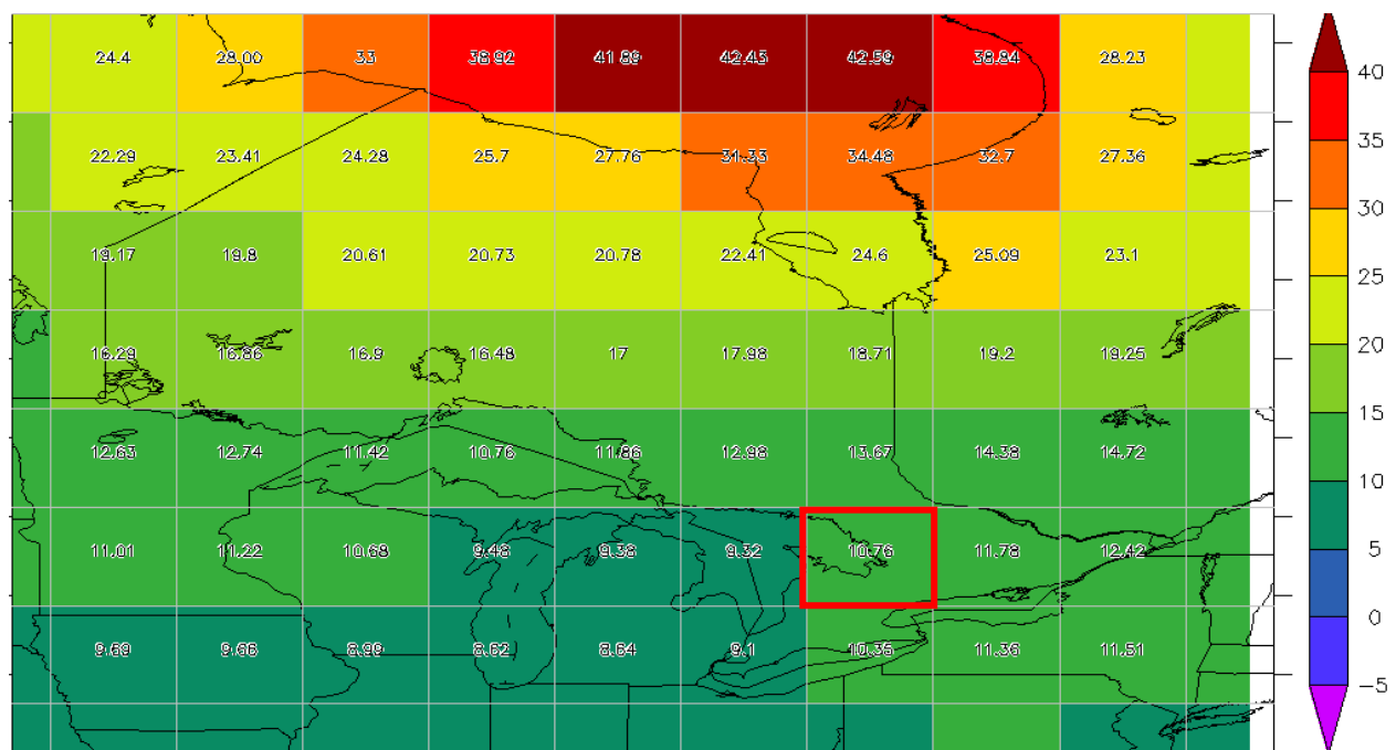
Figure 20-6: Projected change in average WINTER precipitation over Ontario for 2050s compared with 1961-1990 under HIGH GHG emissions (CCCSN, 2009). Area highlighted in red roughly corresponds to the Source Protection Region.
