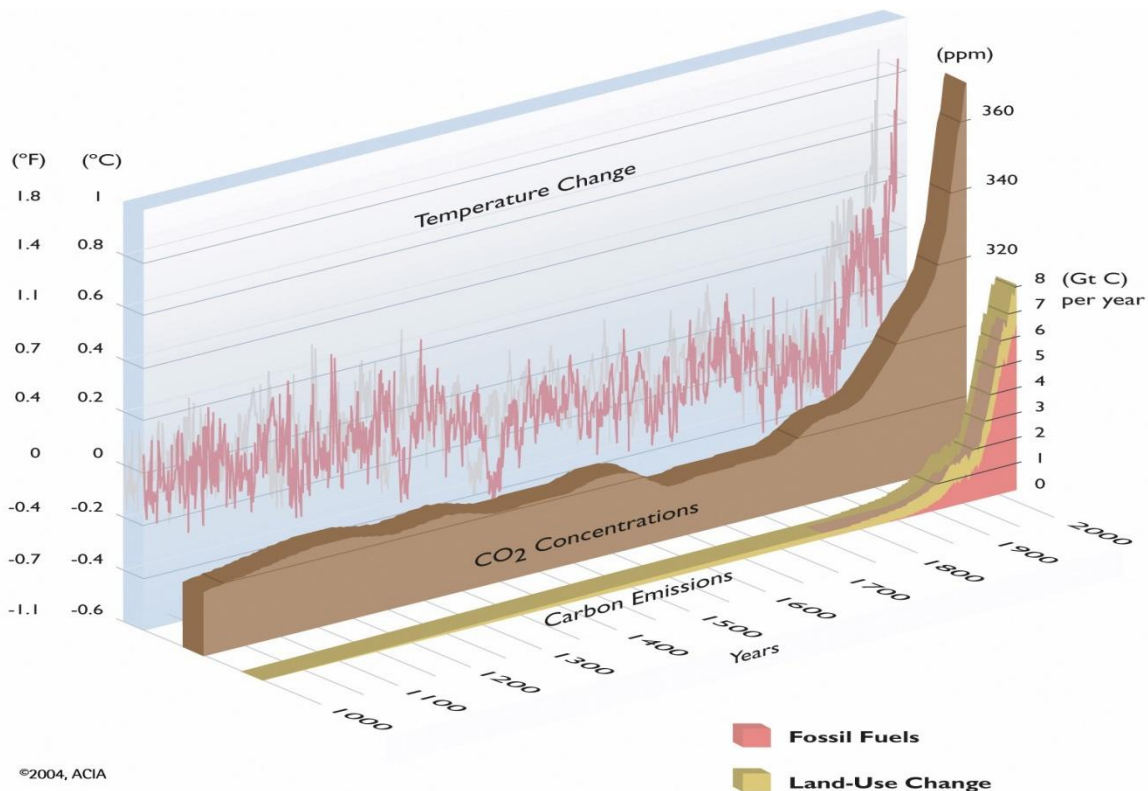
Figure 20-1: Atmospheric Carbon Dioxide and Temperature Change (Peltier, 2007).
