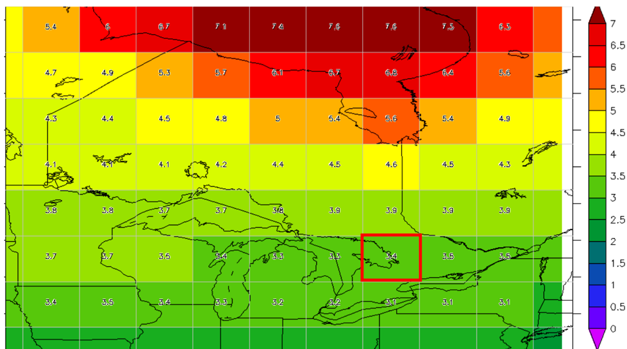
Figure 20-3: Projected change in average WINTER air temperature (°C) over Ontario for 2050s compared with 1961-1990 under HIGH GHG emissions. (CCCSN, 2009). Area highlighted in red roughly corresponds to the Source Protection Region.
