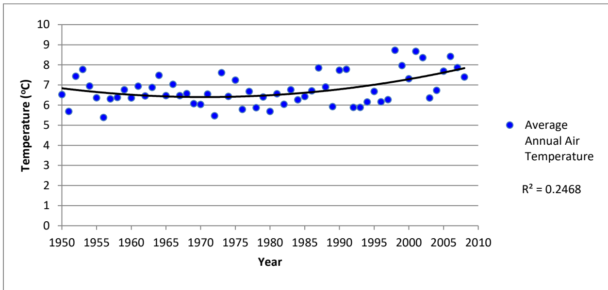
Figure 20-12 : Average Annual Temperature at the Barrie WPCCC Meteorological Monitoring Station
