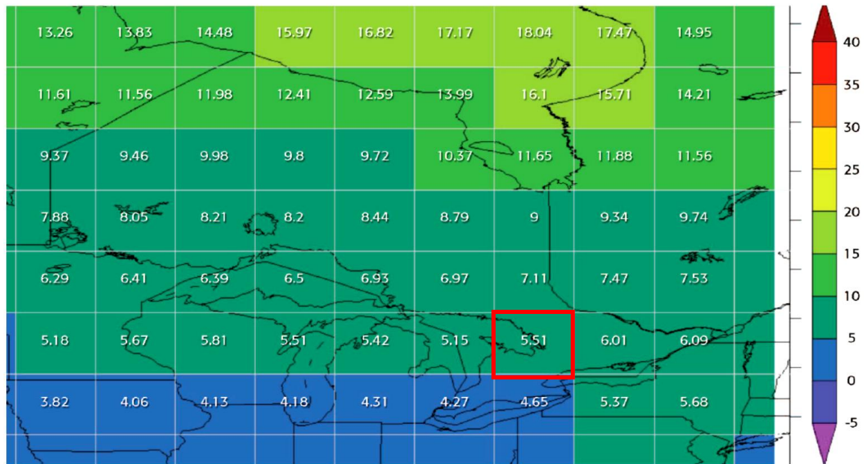
Figure 20-5: Projected change in annual average precipitation (%) over Ontario for 2050s compared with 1961-1990 under HIGH GHG emissions (CCCSN, 2009). Area highlighted in red roughly corresponds to the Source Protection Region.
