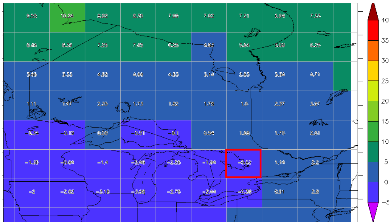
Figure 20-7: Projected change in average SUMMER precipitation over Ontario for 2050s compared with 1961-1990 under HIGH GHG emissions (CCSN, 2009). Area highlighted in red roughly corresponds to the Source Protection Region.
