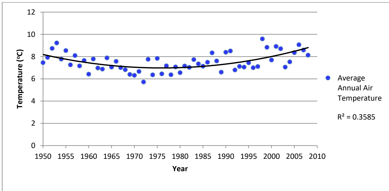
Figure 20-10: Average Annual Temperature at the Alliston-Nelson Meteorological Monitoring Station.
